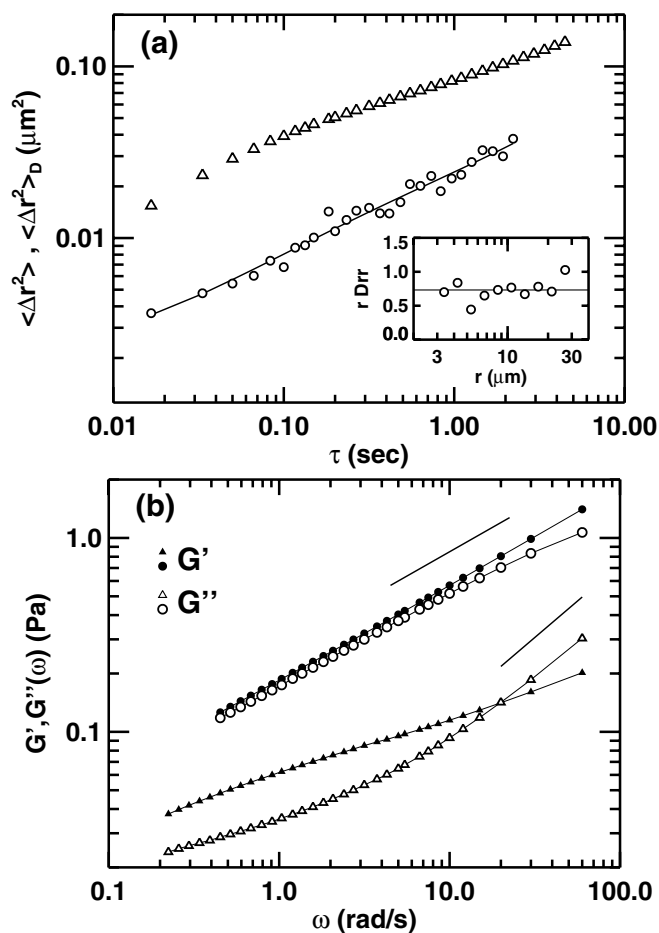
FIG. 3. Comparison of the self (triangles) and distinct (circles) displacements of 0.47 \mu\text{m} diameter beads in a 1 \text{ mg/ml} F-actin solution. The inset shows the r dependence of r D_{rr} for \tau = 67 \text{ msec} , in units of 10^{-3} \mu\text{m}^3 . (b) The storage (filled circles) and loss (open circles) moduli calculated using \langle \Delta r^2(\tau) \rangle_D vary as \omega^{1/2} . The moduli calculated with \langle \Delta r^2(\tau) \rangle (triangles) show a different form approaching \omega^{3/4} . The short lines indicate slopes of 1/2 and 3/4 .
