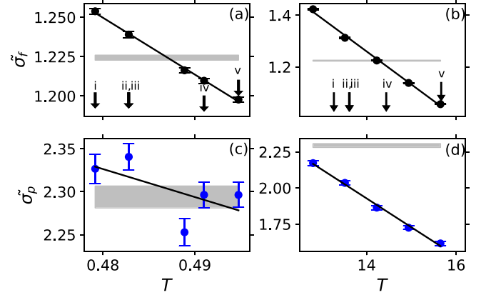
FIG. 4. The reduced flow stress \tilde{\sigma}_f and reduced peak stress \tilde{\sigma}_p against temperature near the point of matching stress at \rho_1 = 1.301 (left two panels) and \rho_9 = 2.789 (right two panels). Glasses cooled (at lowest density) at rate R_{c,0} = 10^{-5} and sheared at reduced strain rate \dot{\epsilon} = 10^{-3} . Solid black lines are linear fits. Gray horizontal lines indicate \tilde{\sigma}_f in panels (a) and (b), and \tilde{\sigma}_p in panels (c) and (d) at the reference density with shaded region indicating error. Arrows in panels (a) and (b) point to T estimated using: (i) DIC stress method; (ii) DIC PE method; (iii) WU/analytic; (iv) FMMOD; (v) FM.
