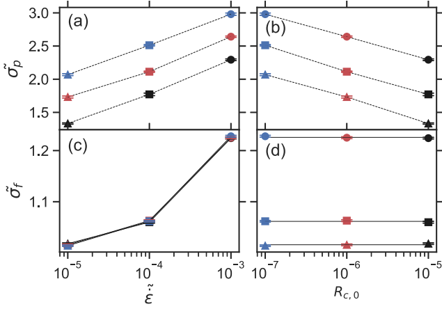
FIG. 13. Reduced peak stress \bar{\sigma}_p and flow stress \bar{\sigma}_f as function of reduced strain rate \tilde{\epsilon} (a, c) and cooling rate R_{c,0} (b, d). Black, red, and blue are for R_{c,0} = 10^{-5}, 10^{-6}, 10^{-7} ; sphere, square, and up triangle are for \tilde{\epsilon} = 10^{-3}, 10^{-4}, 10^{-5} . The flow stress \bar{\sigma}_f is within errors independent of R_{c,0} but increases with \tilde{\epsilon} . See the text for a discussion of the uncertainties of these measurements, which for these data are smaller than the symbol size. The three horizontal lines in panel (d) are the average of the corresponding three points of the same \tilde{\epsilon} .
