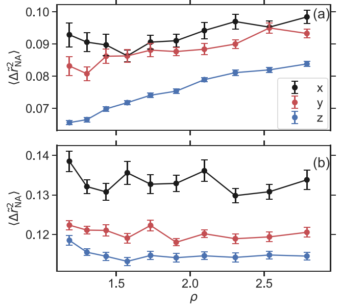
FIG. 10. Comparison of nonaffine particle motion over 12%-strain intervals between (a) transient state with \epsilon \in [0, 0.12] and (b) steady state with \epsilon \in [3.65, 3.77] . Data is averaged over all particles and 40 independent runs. Color indicates the three components of the nonaffine motion squared and shown in the legend in panel (a).
