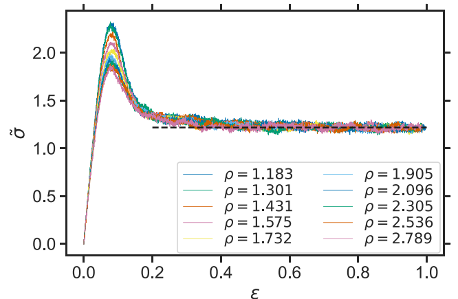
FIG. 6. Reduced stress-strain curves along isomorph determined by the procedure illustrated in Fig. 5. Glasses cooled (at lowest density) at rate R_{c,0} = 10^{-5} and sheared at reduced strain rate \dot{\epsilon} = 10^{-3} .
