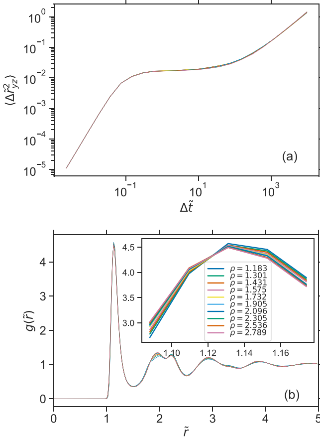
FIG. 9. Collapse of (a) \langle \Delta \tilde{r}_{yz}^2(\tilde{t}) \rangle and (b) g(\tilde{r}) (for AA pairs) for steady state only along an isomorph containing 10 points in the phase diagram calculated using the method described in Sec. IV B. The starting configuration is at \rho_0 = 1.183 and T_0 = 0.3 and was cooled with R_{c,0} = 10^{-5} . Shearing for all state points was with reduced strain rate \tilde{\epsilon} = 10^{-4} . The inset in panel (b) shows a close-up of the first peak.
