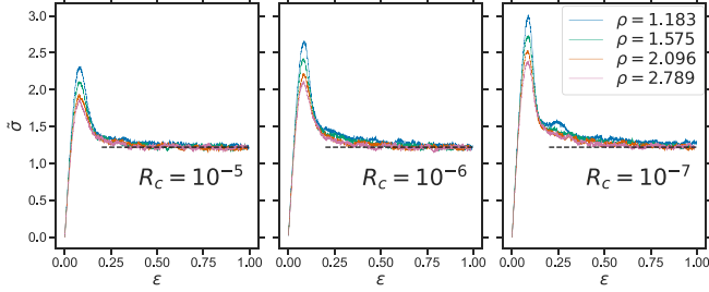
FIG. 15. Stress and strain curves of glasses cooled at three rates and sheared at reduced strain rate \dot{\epsilon} = 10^{-3} . We only show strain up to 1 so that the peak is more visible; only four densities are shown for clarity. The black horizontal dashed lines indicate the flow stress. These curves are where the data of Fig. 7 are derived from.
