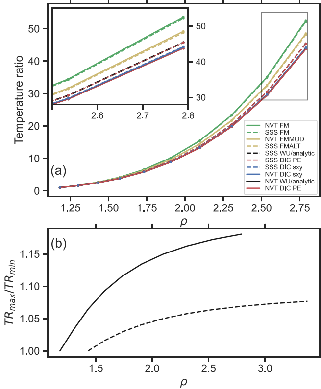
FIG. 3. (a) temperature ratios (TR) from different methods against density for starting density 1.183. Solid lines are for NVT simulation (NVT) 10^7 steps and dashed lines are for steady state (SSS). Inset zooms in for the largest two densities. (b) the ratio between the highest and lowest temperature ratios of the SSS from the top panel versus density. Solid line starts at \rho = 1.183 , and dashed line starts at \rho = 1.301 .
