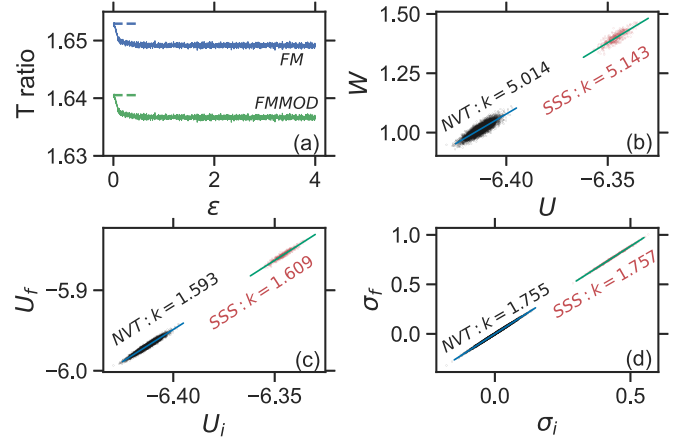
FIG. 2. The five methods to obtain the temperature ratio T_f/T_i used to identify the state point \rho_f, T_f isomorphic to state point \rho_i, T_i from simulations at the latter. The example here uses reference density and temperature \rho_i = 1.183 and T_i = 0.3 and a starting configuration cooled at R_{c,0} = 10^{-5} . We consider a new density \rho_f = 1.1\rho_i = 1.301 . Black indicates results from NVT simulations and red is for the steady state from a shear simulation with the highest (reduced) strain rate \dot{\epsilon} = 10^{-3} . For panels (a), (c), and (d) the system was sampled at regular intervals during the simulation and configurations uniformly scaled to \rho_f ; the potential energy, forces, and shear stress were calculated on the scaled configurations, denoted with subscript f . (a) Temperature ratio given by the force method FM (blue), Eq. (2), and modified force method (green), Eq. (3) from the same shear simulation. The dotted horizontal lines indicate the corresponding temperature ratios from the NVT simulation. (b) Scatter-plot of the virial W versus potential energy U . The slopes (correlation coefficient) of the two fits are 5.014 (0.869) and 5.143 (0.859), respectively, where the slopes can be considered estimates of the density scaling exponent \gamma , which yields the temperature factor via Eqs. (C4) and (C6). (c) Scatter-plot of U_f against U_i (DIC-pe). The slopes (correlation coefficient) are 1.593 (0.975) and 1.609 (0.972), respectively. Here the slopes correspond directly to the temperature ratios. (d) Scatter-plot of \sigma_f against \sigma_i . The slopes (correlation coefficient) are 1.755 (1.00) and 1.757 (0.999). Here the temperature ratio is the slope divided by the density ratio (1.1). Table I gives the results of the different methods.
