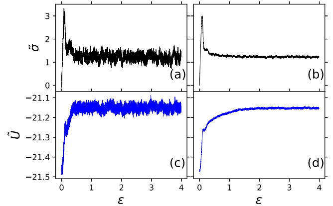
FIG. 1. Examples of reduced-unit shear stress (top panels) and potential energy per particle (bottom panels) versus strain, from shear deformation of a binary Lennard-Jones glass with density 1.183 at temperature 0.3. The glass was prepared by cooling at the rate 10^{-7} (LJ units), while the deformation was carried out at reduced strain rate 10^{-5} , meaning the real strain rate was 10^{-5} \rho^{1/3} (T)^{1/2} \simeq 5.8 \times 10^{-6} . The left panels show curves from a single run, while the right panels show the average of 40 independent runs.
