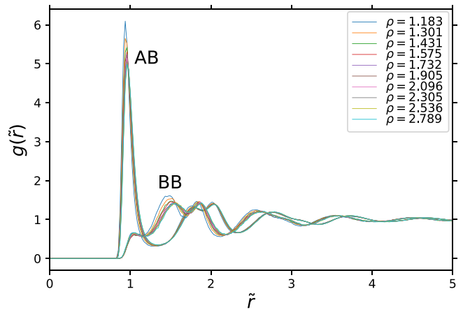
FIG. 18. Collapse of g(\bar{r}) for AB and BB pairs as complement to Fig. 9(b).
