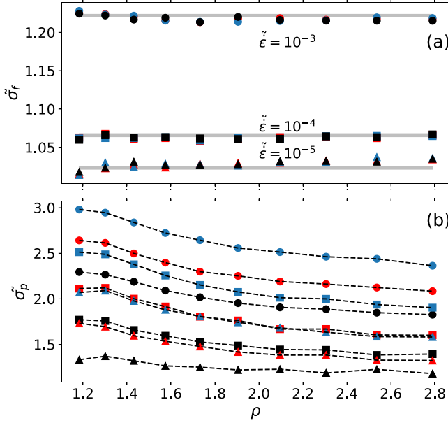
FIG. 7. (a) \sigma_f and (b) \sigma_p against density along the isomorph for R_{c,0} = 10^{-5}, 10^{-6}, 10^{-7} (black, red, blue), and \dot{\epsilon} = 10^{-3}, 10^{-4}, 10^{-5} (circle, square, triangle). Each point in panel (a) is an average of 40 shear simulations (on 40 individual configurations, or 30 for \dot{\epsilon} = 10^{-5} ) and the uncertainties are computed as described in Sec. III B. For the peak stress [panel (b)], we first divide the 40 shear runs into five groups and obtain five averaged stress and strain curves. We then fit the data for 10% strain around the maximum stress using a fourth-degree polynomial and identify the maximum of the fit as the \sigma_p . The error is the standard deviation of the five values divided by \sqrt{5} . The three families in panel (a) correspond to \dot{\epsilon} = 10^{-3}, 10^{-4}, 10^{-5} from top to bottom respectively. The errors are all smaller than the marker size. The position of the gray bars in panel (a) are the reference \sigma_f (at \rho_1 cooled with R_{c,0} = 10^{-5} and sheared with \dot{\epsilon} = 10^{-3} ) and the width of the bar indicates the reference \sigma_f plus or minus the uncertainty.
