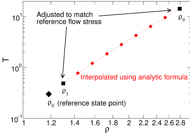
FIG. 5. The isomorph determined by matching flow stress again on glasses cooled (at lowest density) at rate R_{c,0} = 10^{-5} and sheared at \dot{\epsilon} = 10^{-3} . The large black diamond indicates the reference state point. The two black squares represent points whose temperatures were identified by matching the reduced flow stress to that of the reference, using the linear fits in Fig. 4, and the red diamonds are points whose temperatures have been determined by interpolation between the black squares, using Eq. (4).
