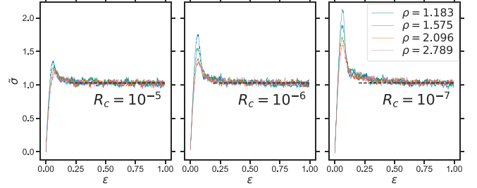
FIG. 17. Same as in Fig. 15 but now for glasses cooled at three rates and sheared at reduced strain rate \dot{\epsilon} = 10^{-5} .
