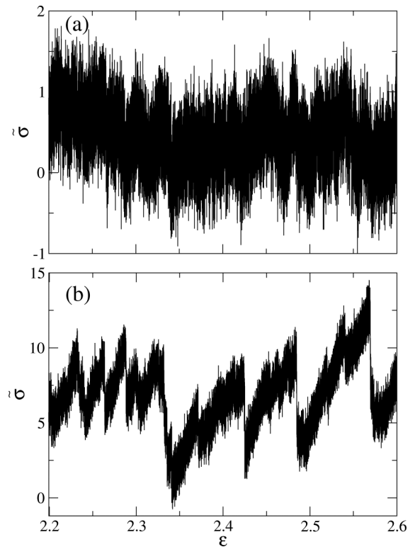
FIG. 3. (a) Section of the stress-strain curve for the lowest-density state point on the higher-temperature isomorph ( \rho = 1.265 , T = 0.550 ) at the lowest nominal strain rate 10^{-5} . (b) Section of the stress-strain curve for a state point on the lower-temperature isomorph ( \rho = 1.324 , T = 0.100 ) at the lowest strain rate 10^{-5} . The abrupt drops can be identified with avalanches of plastic activity. The difference in vertical scale between (a) and (b) can be attributed partly to the definition of reduced units for stress.
