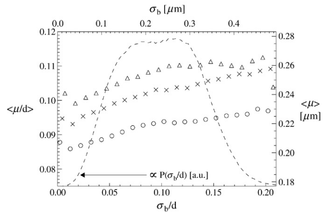
Fig. 6. Average tetrahedral mobility as a function of irregularity \sigma_b/d . The three curves represent three different ages of the sample. \Delta : t_w = 0\tau_{\text{diff}} , \times : t_w = 100\tau_{\text{diff}} and \circ : t_w = 300\tau_{\text{diff}} . The dashed curve represents the distribution P(\sigma_b/d) and is shown here to highlight the lack of statistics at low ( \sigma_b/d < 0.01 ) and high ( \sigma_b/d > 0.2 ) values of \sigma_b/d .
