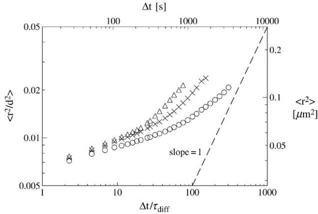
Fig. 1. Aging mean squared displacement for a colloidal glass at \phi \approx 0.62 . The three curves represent three different ages of the sample. \Delta : t_w = 0\tau_{\text{diff}} , \times : t_w = 100\tau_{\text{diff}} and \circ : t_w = 300\tau_{\text{diff}} . The dashed line has a slope of 1 and represents diffusive behavior, not seen in this glassy sample.
