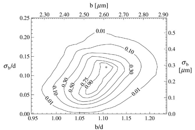
Fig. 3. Contour plot showing the abundance of tetrahedra with a given looseness and irregularity. The iso-curves are labeled relative to the peak tetrahedral abundance at \{b/d = 1.11; \sigma_b/d = 0.12\} .
