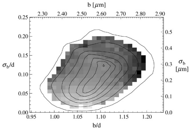
Fig. 4. Plot of tetrahedral mobility ( \langle \mu \rangle (\Delta t = 50\tau_{\text{diff}}) ), averaged over all ages, versus looseness b/d and irregularity \sigma_b/d . The darker the color the more mobile the tetrahedron. The contour lines are the same as in Fig. 3 and represent the abundance of tetrahedra with a given value of b/d and \sigma_b/d .
