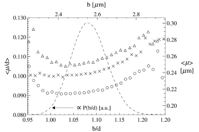
Fig. 5. Average tetrahedral mobility as a function of looseness b/d . The three curves represent three different ages of the sample. \Delta : t_w = 0\tau_{\text{diff}} , \times : t_w = 100\tau_{\text{diff}} and \circ : t_w = 300\tau_{\text{diff}} . The dashed curve represents the distribution P(b/d) and is shown here to highlight the lack of statistics at low ( b/d < 0.98 ) and high ( b/d > 1.2 ) values of b/d .
